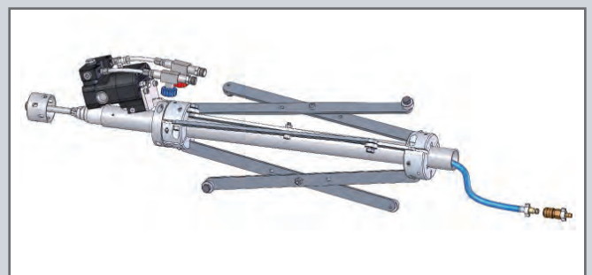
PU 4040 Automatic Gun for internal pipe coating with Polyurea Orde No. 0659289 • Guide ø 210- ø 400 mm (Larger dia. upon request)
